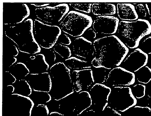
— 10 \mu\text{m} 3.0 kV X 500 11mm
